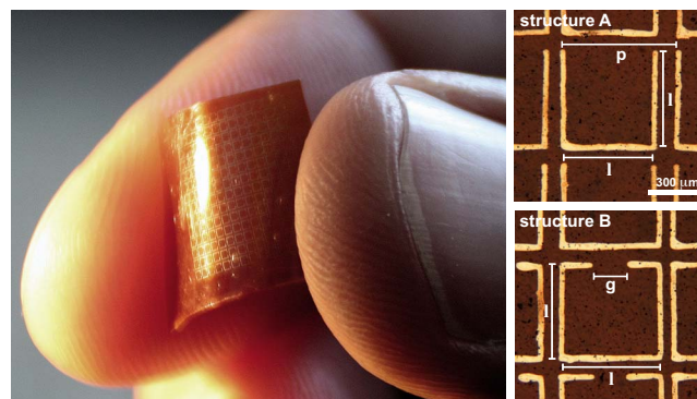
FIG. 1. (Color online) Inkjet printed SRR arrays on a flexible polyimide substrate. Two different structures have been fabricated ( l=500 \mu\text{m} , p=600 \mu\text{m} , g=200 \mu\text{m} ).
